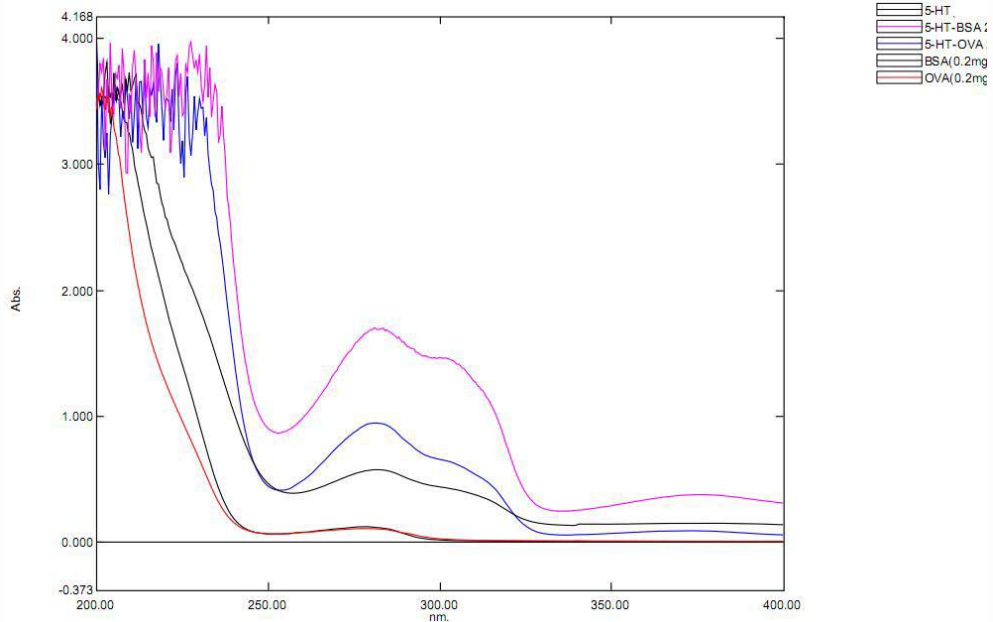
Figure 2. UV-spectrum
